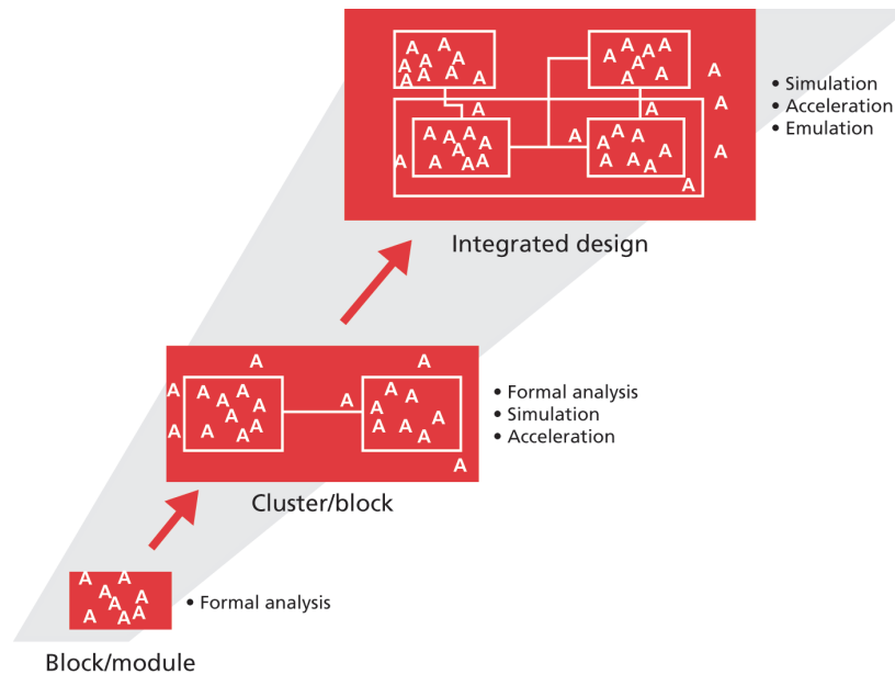
Figure 2: Formal analysis at the entry point of the Incisive platform's complete assertion-based verification flow
