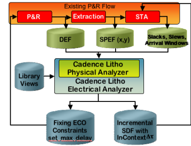
Place-and-route flow
