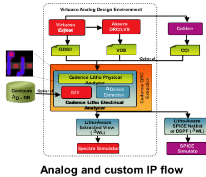
Analog and custom IP flow
